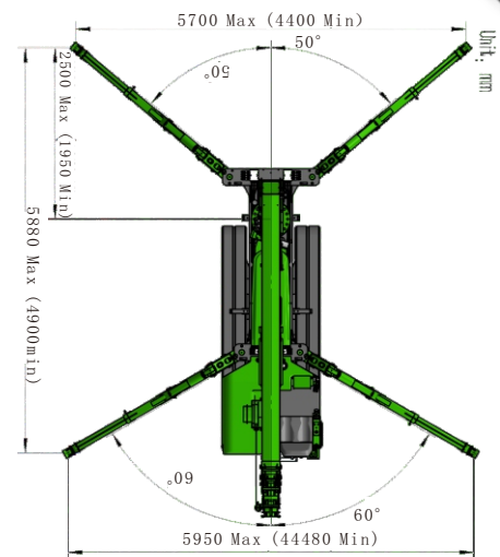
Outrigger Footprints
