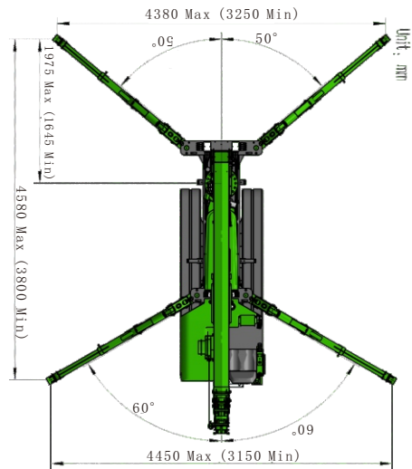
Outrigger Footprints
