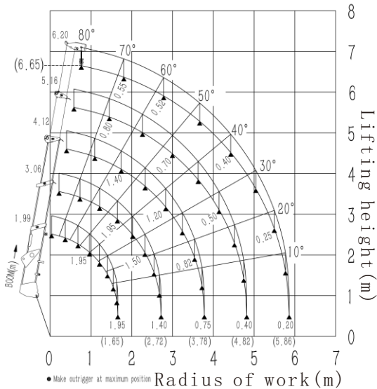
Working Range Diagram
