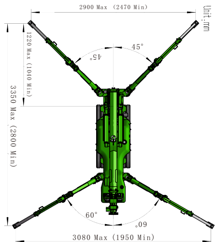
Outrigger Footprints
